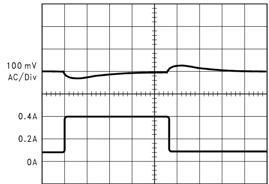
Load Transient Response for Discontinuous Mode V_{IN} = 20V , V_{OUT} = 5V , L = 47\text{ }\mu\text{H} , C_{OUT} = 68\text{ }\mu\text{F} , C_{OUT}ESR = 50\text{ m}\Omega
