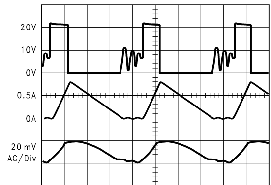
Discontinuous Mode Switching Waveforms V_{IN} = 20V , V_{OUT} = 5V , I_{LOAD} = 300\text{ mA} L = 15\text{ }\mu\text{H} , C_{OUT} = 68\text{ }\mu\text{F} (2x), C_{OUT}ESR = 25\text{ m}\Omega
