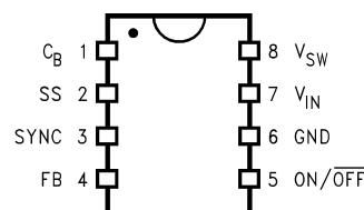
SO-8/DIP Package
