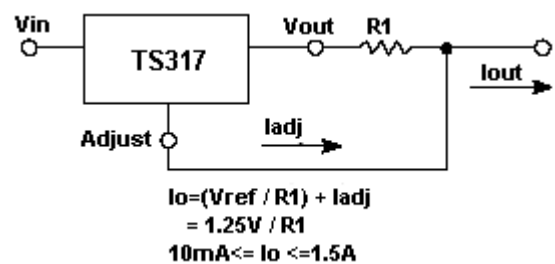
Figure 11. current regulator
