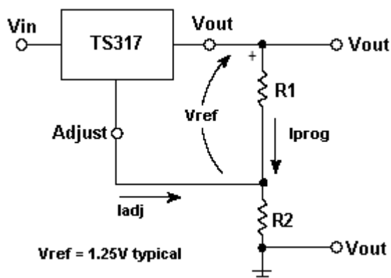
Figure 5. basic circuit configuration
