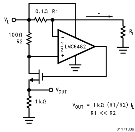
FIGURE 22. Positive Supply Current Sense
