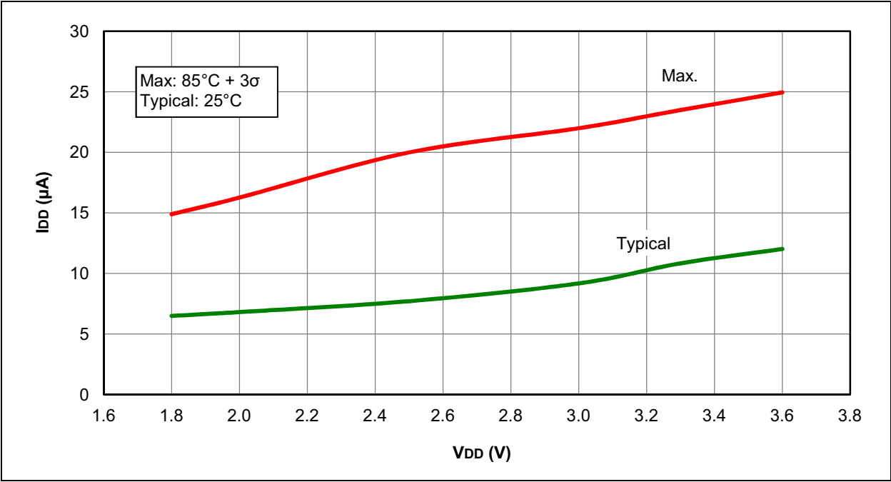
FIGURE 31-19: I DD , LFINTOSC, F osc = 31 kHz, PIC12LF1840 ONLY
