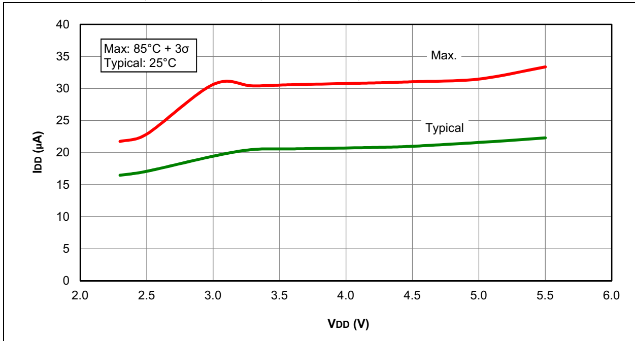
FIGURE 31-2: I_{DD} , LP OSCILLATOR, F_{osc} = 32 kHz, PIC12F1840 ONLY
