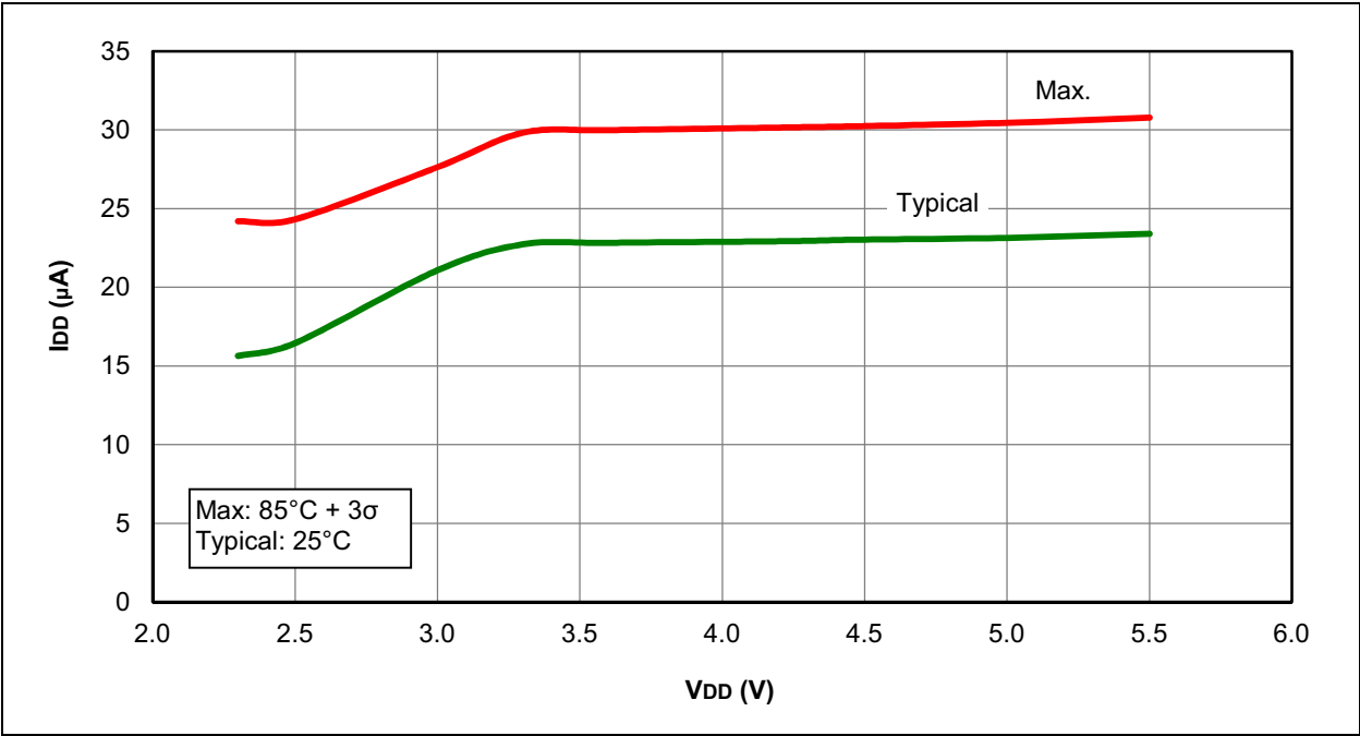
FIGURE 31-20: I DD , LFINTOSC, F osc = 31 kHz, PIC12F1840 ONLY
