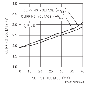
Clipping Voltage vs Supply Voltage
