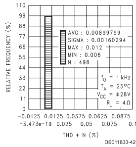
THD + N Distribution
