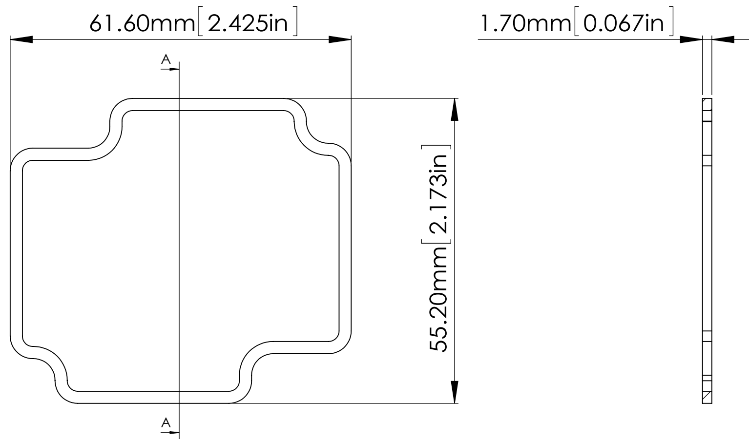
SECTION A-A SCALE 1.5:1
