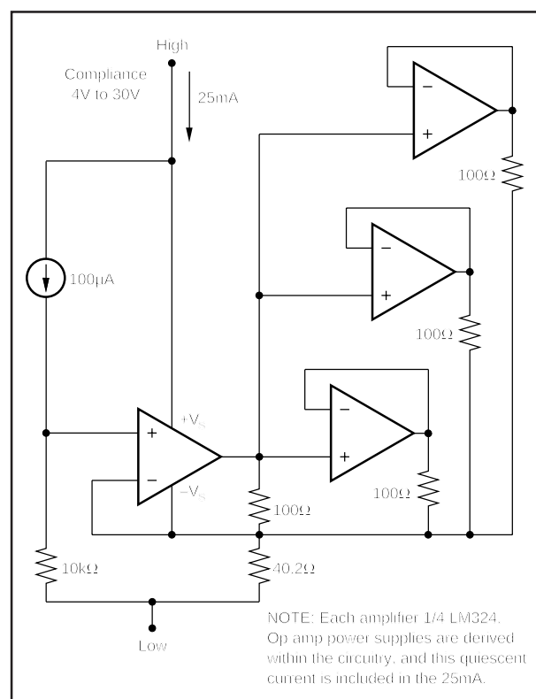
FIGURE 18. 25mA Floating Current Source.
