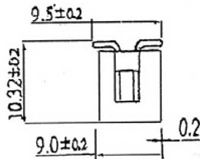
( SMT Type )
