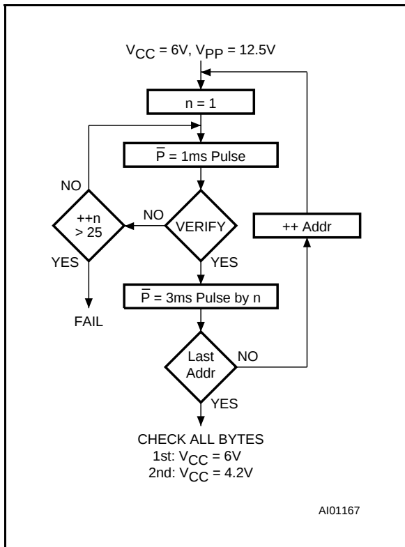
Figure 7. Programming Flowchart
