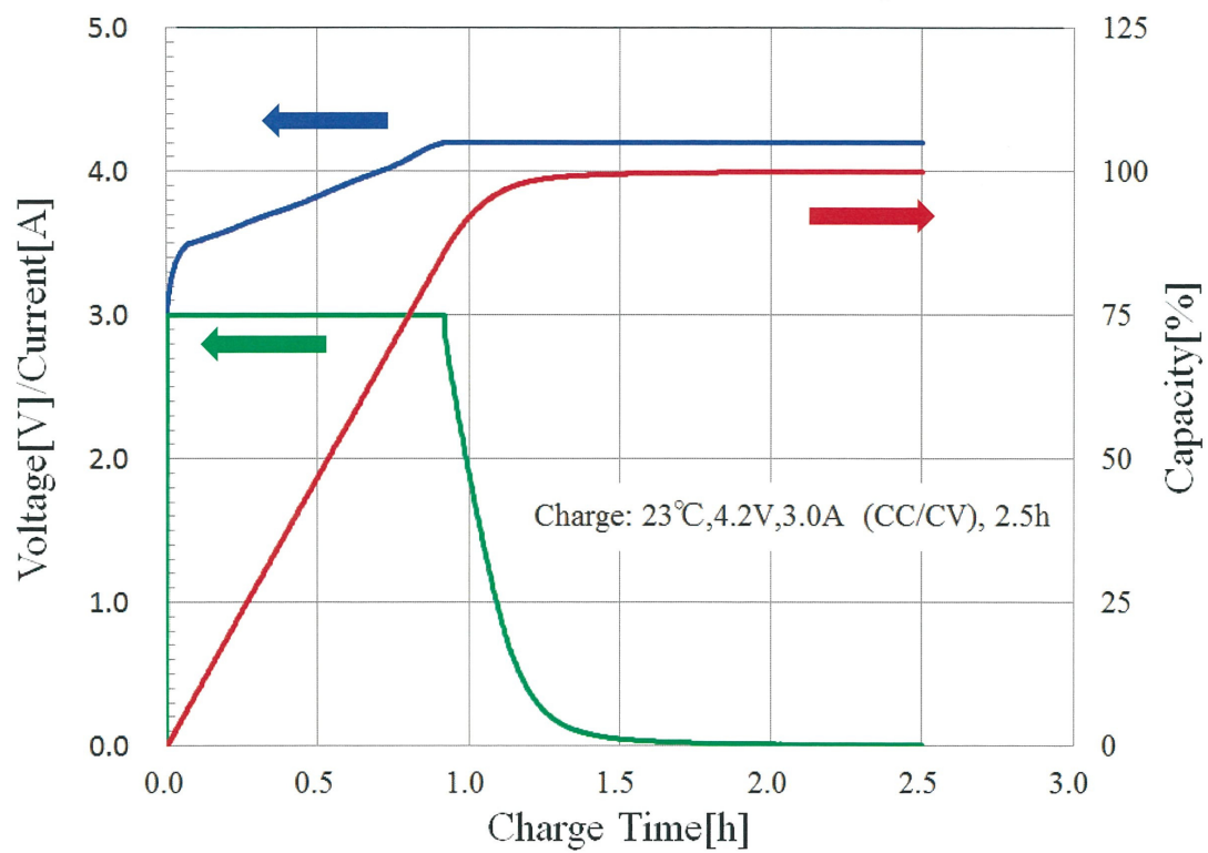
Charge Characteristics (US18650VTC6)
