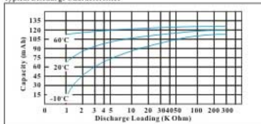
Typical Discharge Characteristics
