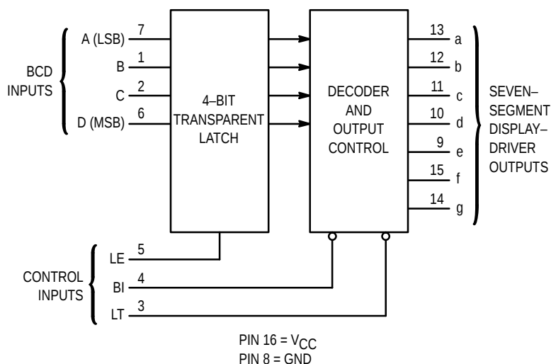
LOGIC DIAGRAM
