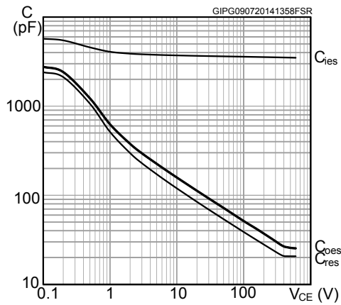
Figure 13. Capacitance variations
