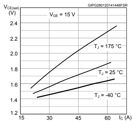
Figure 6. V_{CE(sat)} vs collector current
