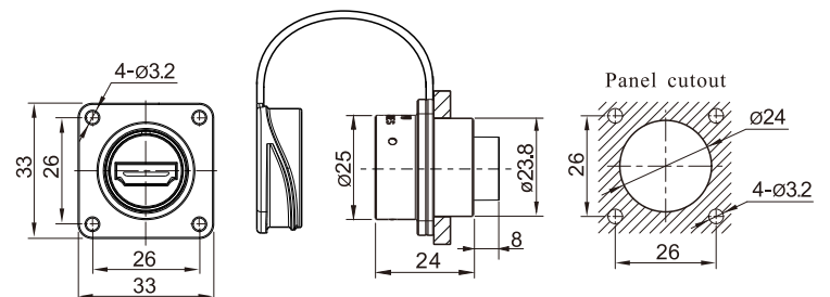
HDMI2.0 Square flange receptacle Mate with SA2410
