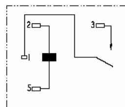
SPST-NO
