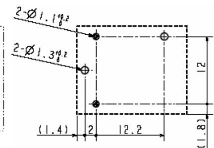
SPST-NO
